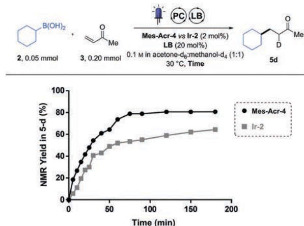
Fig. 1 Reaction following of Mes-Acr-4 against Ir-2 in NMR tube. Reaction monitoring using 1 H-NMR, comparison between Mes-Acr-4 (dots) and Ir-2 (squares). Reactions carried out at 0.05 mmol of 2, 0.2 mmol of 3, 2 mol% of the indicated PC and 20 mol% DMAP in deuterated solvents.
